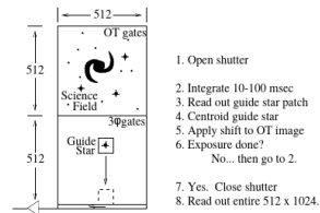
Fig. 2.— The OTCCD is used to track image motion by placing the science field on the portion of the CCD with OT gates and a guide star on the frame-store portion of the CCD. A
